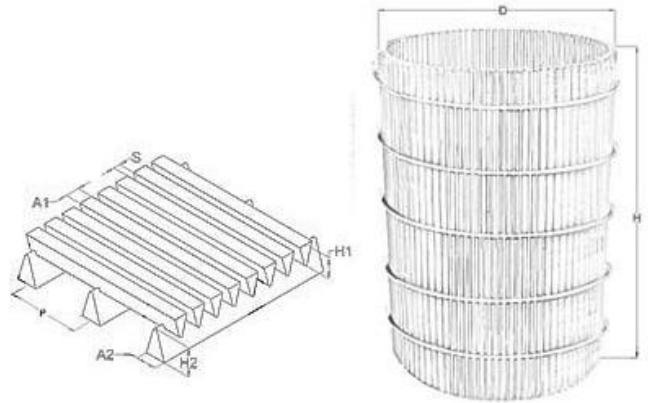
Wedge Wire Cylindrical Screen
