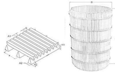
Wedge Wire Cylindrical Screen
