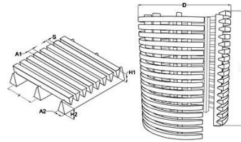
Reverse formed wedge wire screen pipe
