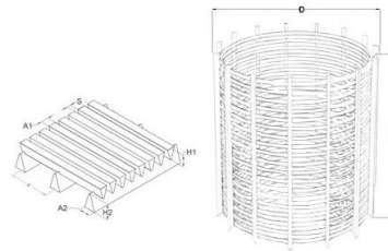
Reverse formed wedge wire screen pipe
