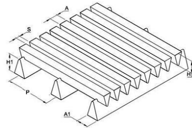
Sieve Bend Screen
