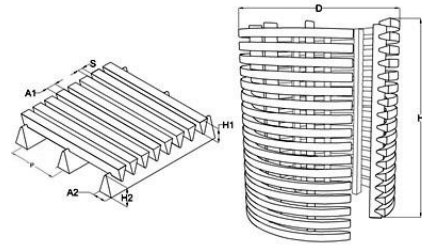
Wedge Wire Cylindrical Screen
