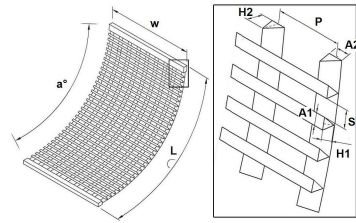
Sieve Bend Screen
