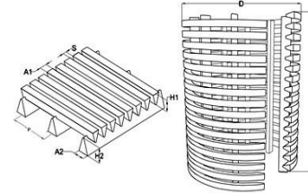
External Circumferential Wire and Axial Internal Support Rods
