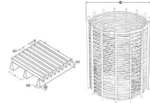
Internal Circumferential Wire with External Axial Support Rods
