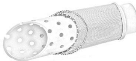
Pre-pack Wrapped Sand Control Screen
