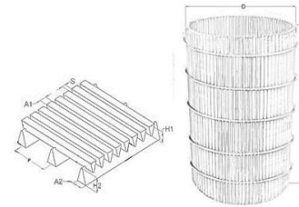
Internal Axial Wire with External Circumferential Support Rods
